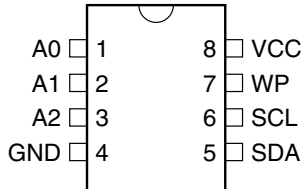
8-pin PDIP
